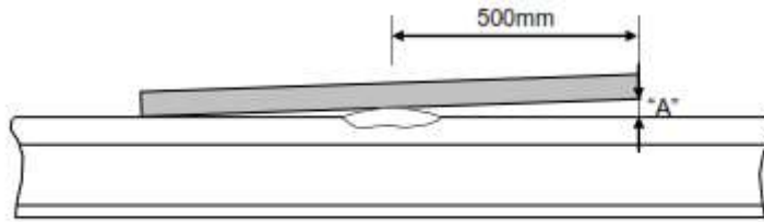
Figure 13 – Head Repair misalignment tolerance in vertical plane (peaking)
